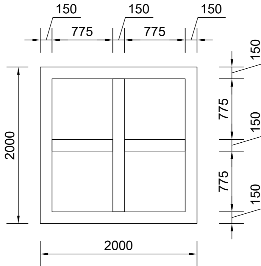
TANK BASE_BLOCK Scale - NTS
