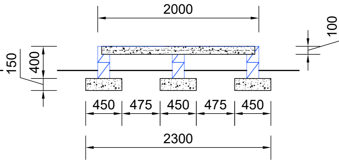
TANK BASE_SECTION Scale - NTS
